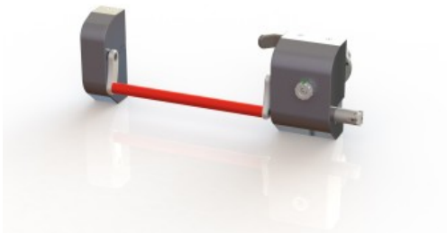
New anti-panic lock with self-locking bolt
