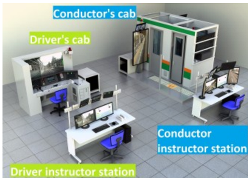
Simulator system for training train personnel
