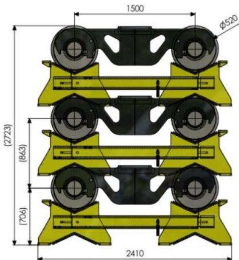
Wheelbase adjustable stacking racks as ideal solution for space-saving bogie storage
