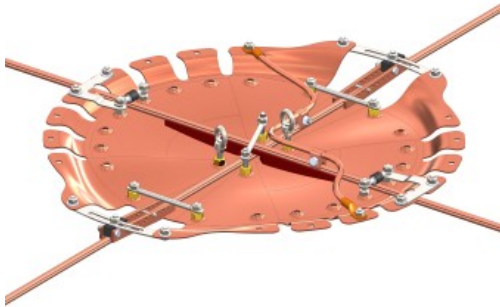
The new contact wire crossing (design modifications are reserved)
