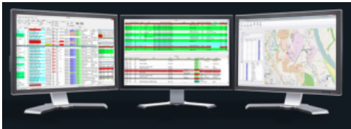
Multi-criteria optimization
